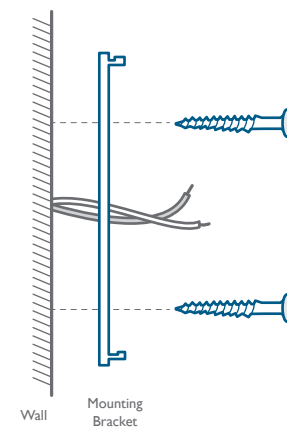
Without 15° Mounting Wedge
